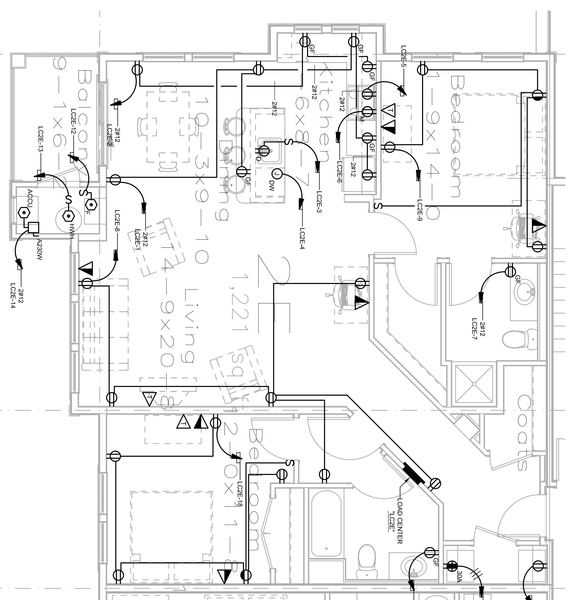
UNIT '2E' ELECTRICAL PLAN SCALE: 1/4" = 1'-0"
