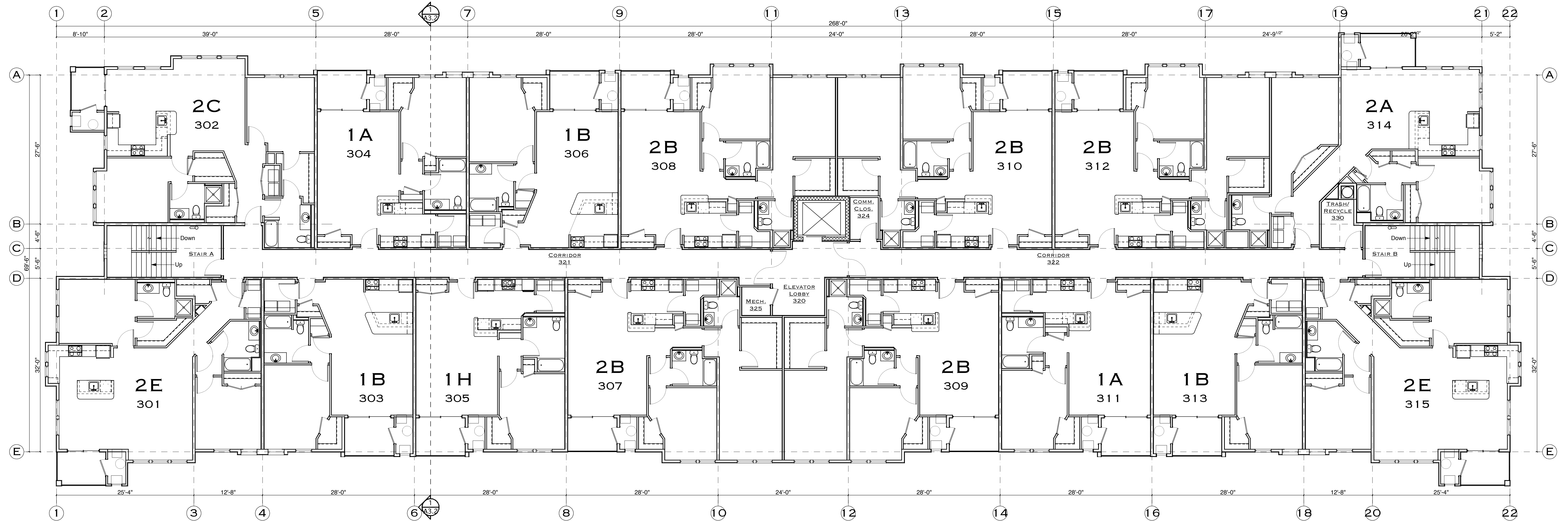
2 Third Floor Plan A1.2 Scale 1/8" = 1'-0"
